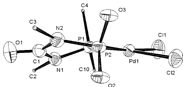
Figure 2. Central metallacycle in 1 and adjacent atoms.
